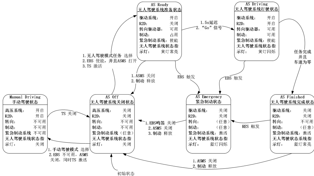
图 4.2 AS 状态机
