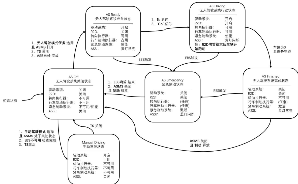
图 4.2 AS 状态机
