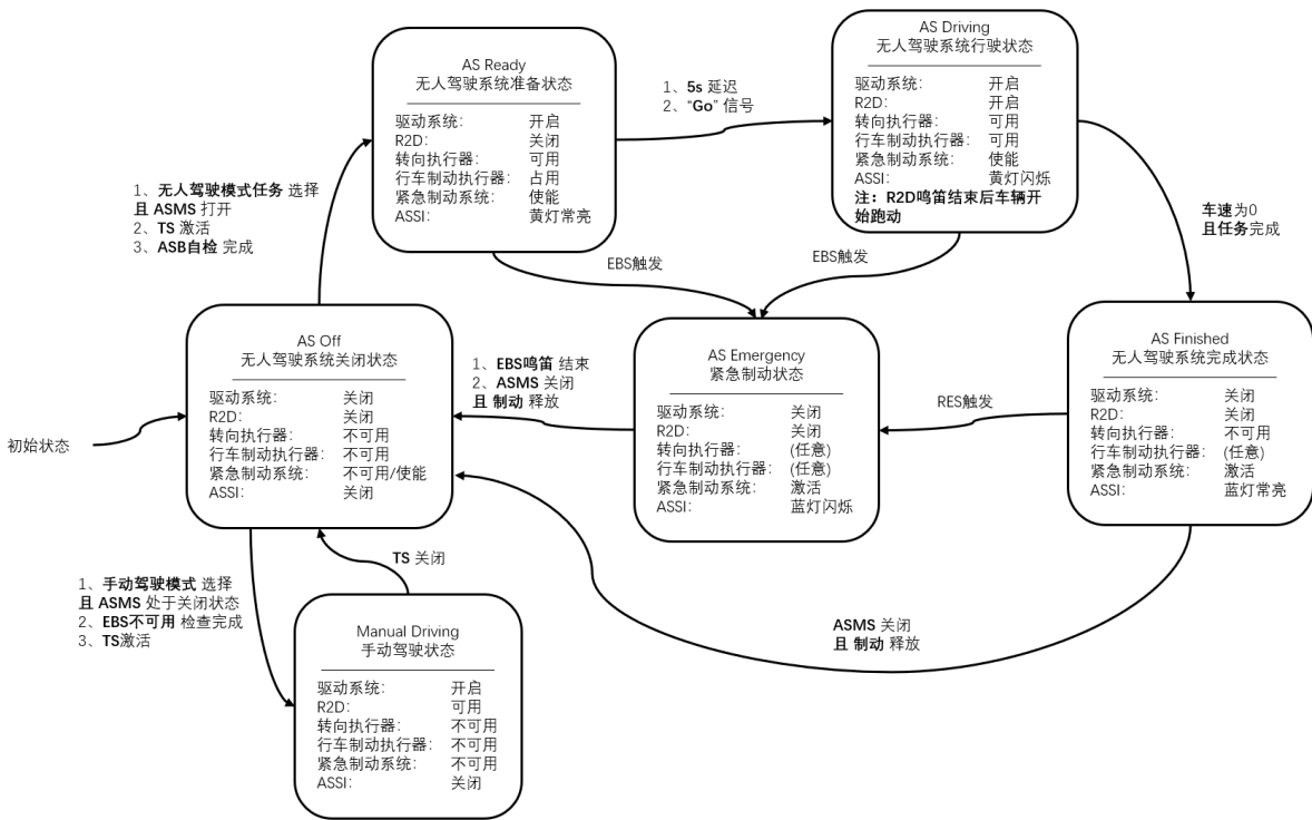
图 4.2 AS 状态机
